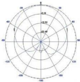
Horizontal plane pattern
